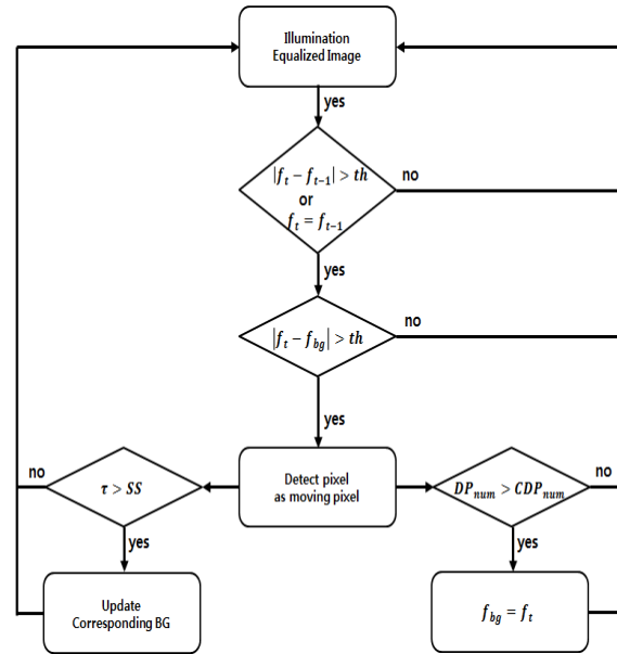
Fig. 1 Moving object detection with dynamic background change
