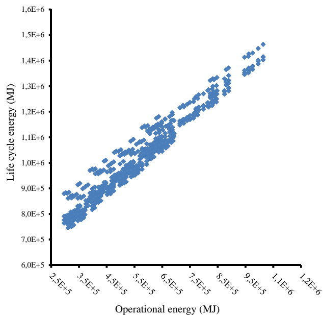
Fig. 2 Operational energy vs life cycle energy
