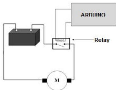
Fig. 13 Transmission Module
