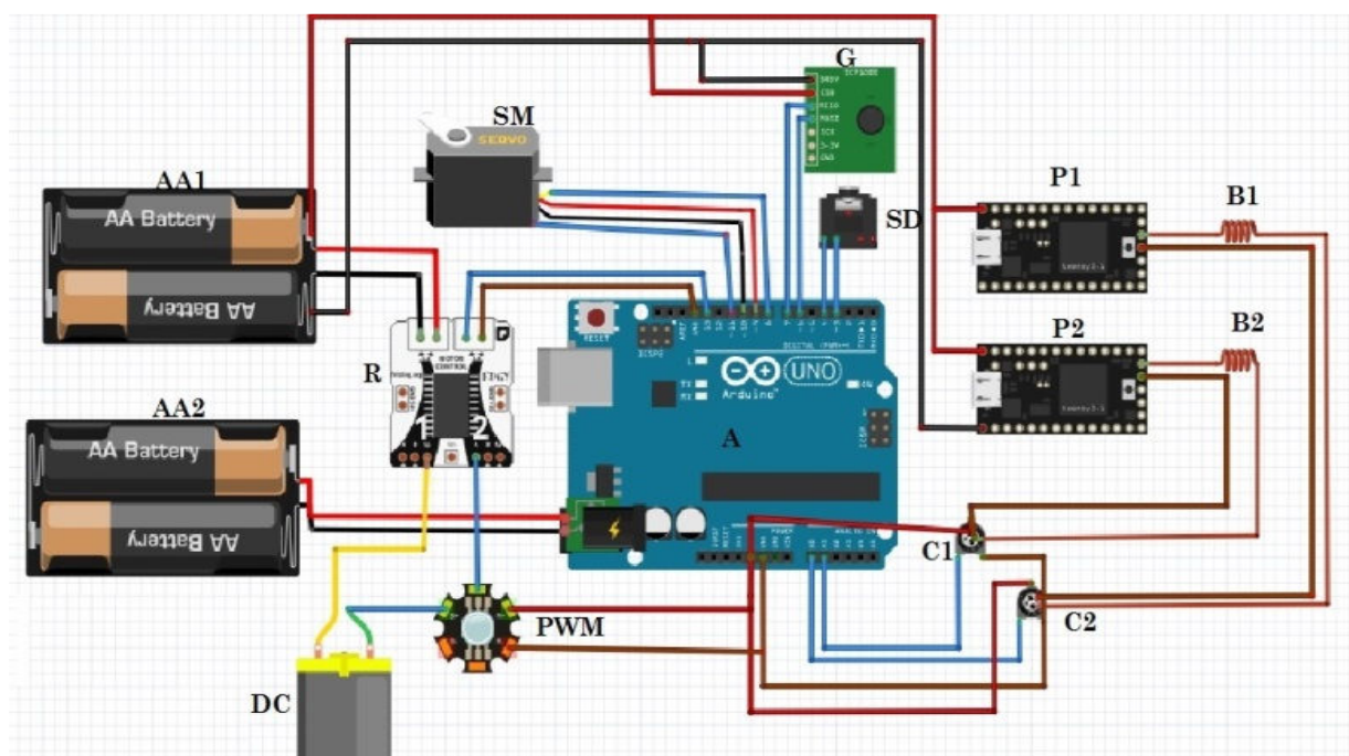
Fig. 17 Electric Circuit Diagram
