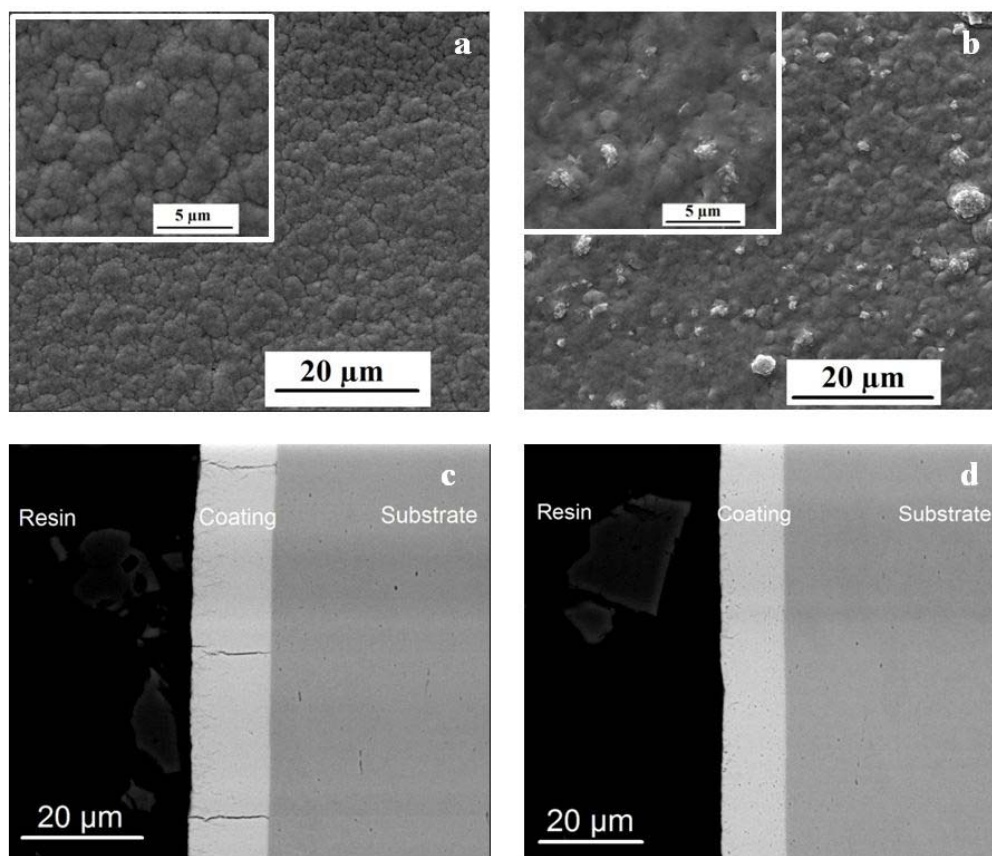
Fig. 5 ESEM images of a) Zn-Ni coating, b) Zn-Ni-Al 2 O 3 coating, and cross-section images of c) Zn-Ni coating d) Zn-Ni-Al 2 O 3 coating
