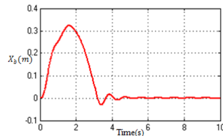
Fig. 5 Passive suspension travel
