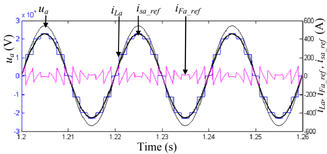
Fig. 7 Supply voltage, load current, reference compensating current and resulted supply current after compensation, when APF is connected in the transformer primary of a traction substation with 12 pulse parallel rectifier
