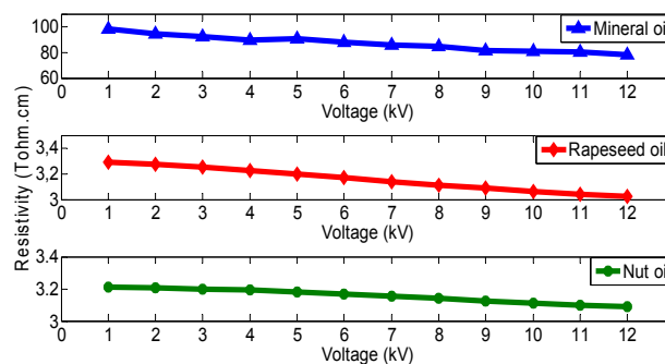
Fig. 4 Change of resistivity with voltage
