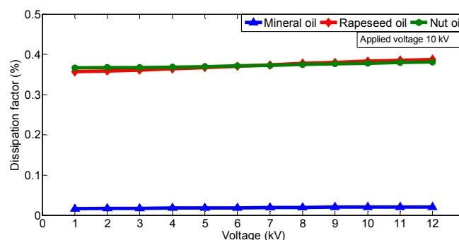
Fig. 1 Change of tan delta depending on voltage
