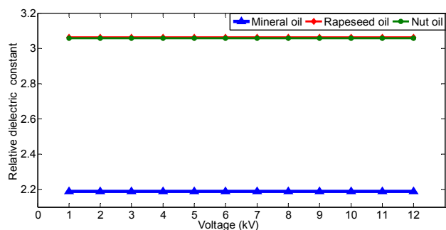
Fig. 3 Change of relative dielectric constant with voltage
