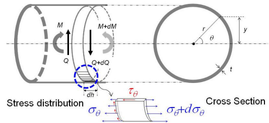
Fig. 3 Stress distribution on the infinitesimal length
