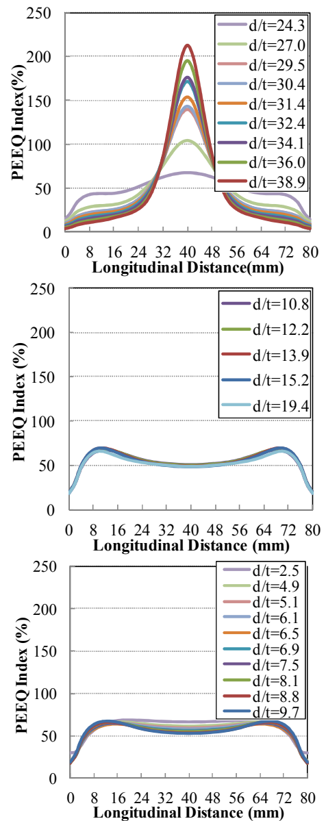
Fig. 12 Equivalent plastic strain measured longitudinally
