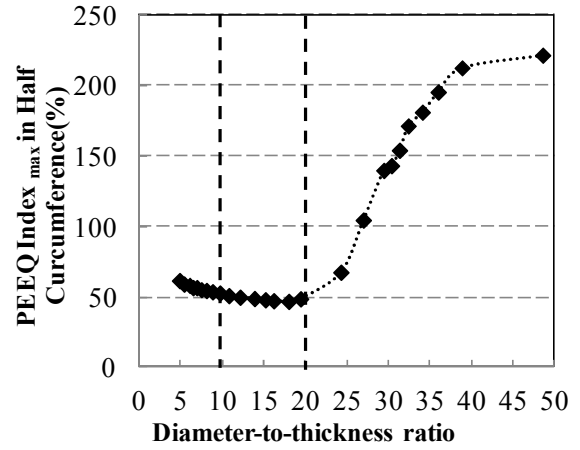
Fig. 11 Circumference PEEQ Index- d/t relationship
