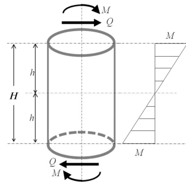
Fig. 1 Loading condition
