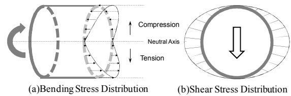
Fig. 2 Stress distribution on CHS Damper
