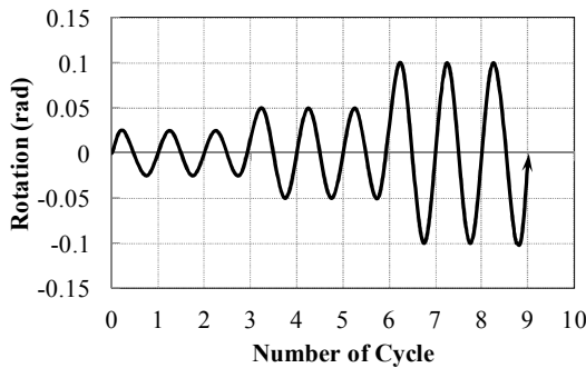
Fig. 6 Loading protocol
