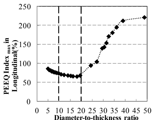
Fig. 13 Longitudinal PEEQ Index- d/t relationship
