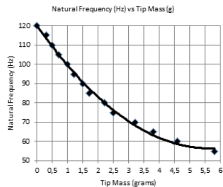
Fig. 7 Results from bandwidth tuning for the PZT cantilever bimorph using tungsten mass
