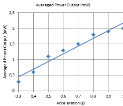
Fig. 10 Average power output (μW) across series of acceleration (g)
