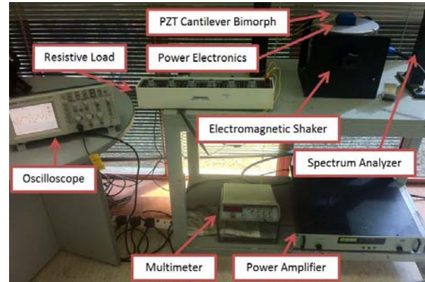
Fig. 5 Experiment configuration for validation purposes
