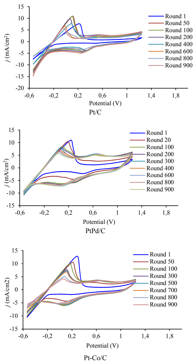
Fig. 4 CV curves of the as-prepared electrocatalysts at a metal loading of 0.15 mg/cm^2 after the indicated number of round of sequential potential cycling in 0.5 M H_2SO_4 at a scan rate of 20 mV/s
