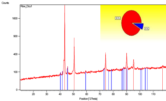
Fig. 8 (a) XRD pattern of Cu-3.5wt%Ti aged at 500°C for 8hr after 50% cold work
