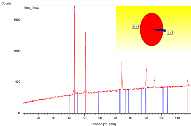
Fig. 8 (b) XRD pattern of Cu-1.5wt%Ti aged at 600°C for 4hr after 50% cold work
