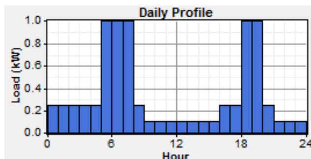
Fig. 4 Average hourly load profile
