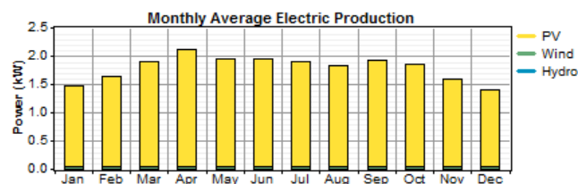
Fig. 7 Average monthly power generation
