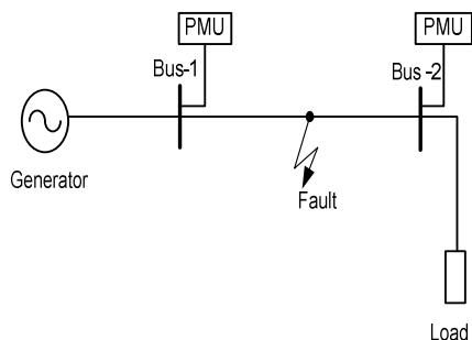
Fig. 2 Single Line Diagram of Two Bus Power System Network with PMUs
