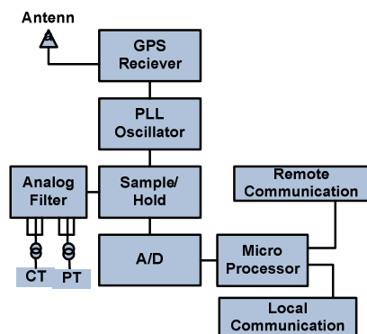
Fig. 1 Phasor Measurement Unit Architecture
