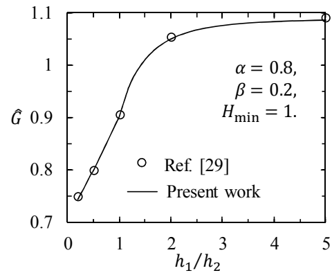
Fig. 3 Normalized ERR vs. layer thickness ratio
