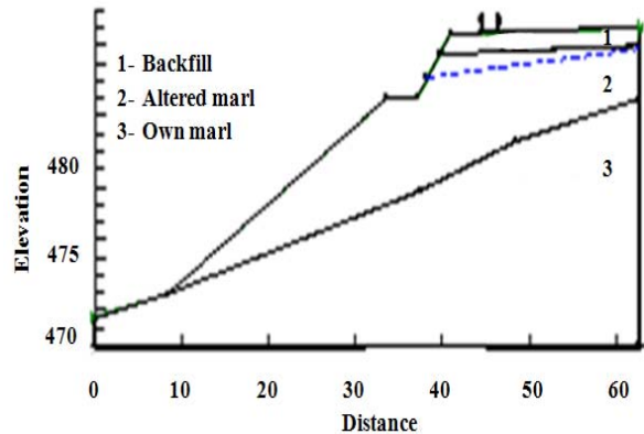
Fig. 1 General configuration of the analyzed slope
