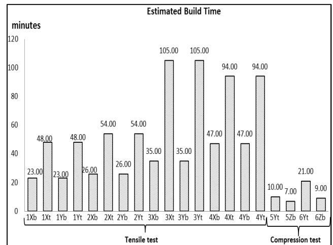
Fig. 8 Estimated build time of specimens
