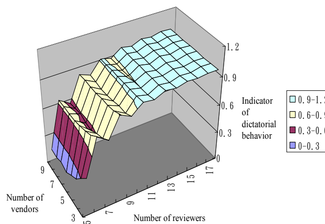
Fig. 2 Test results for ranking method Non-dictatorship
