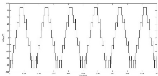
Fig. 11 Output voltage for 9-level CHBMLI by SPWM
