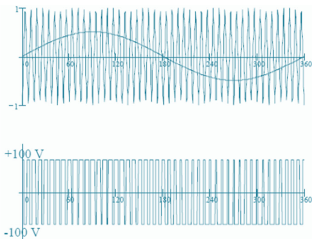
Fig. 4 SPWM with f_c/f_m
