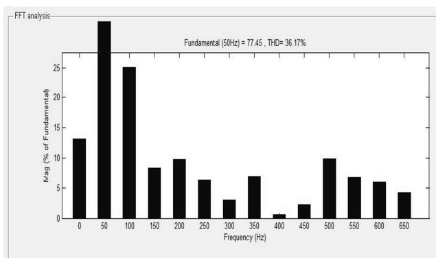
Fig. 12 Harmonic spectrum of 9-level CHBMLI by SPWM
