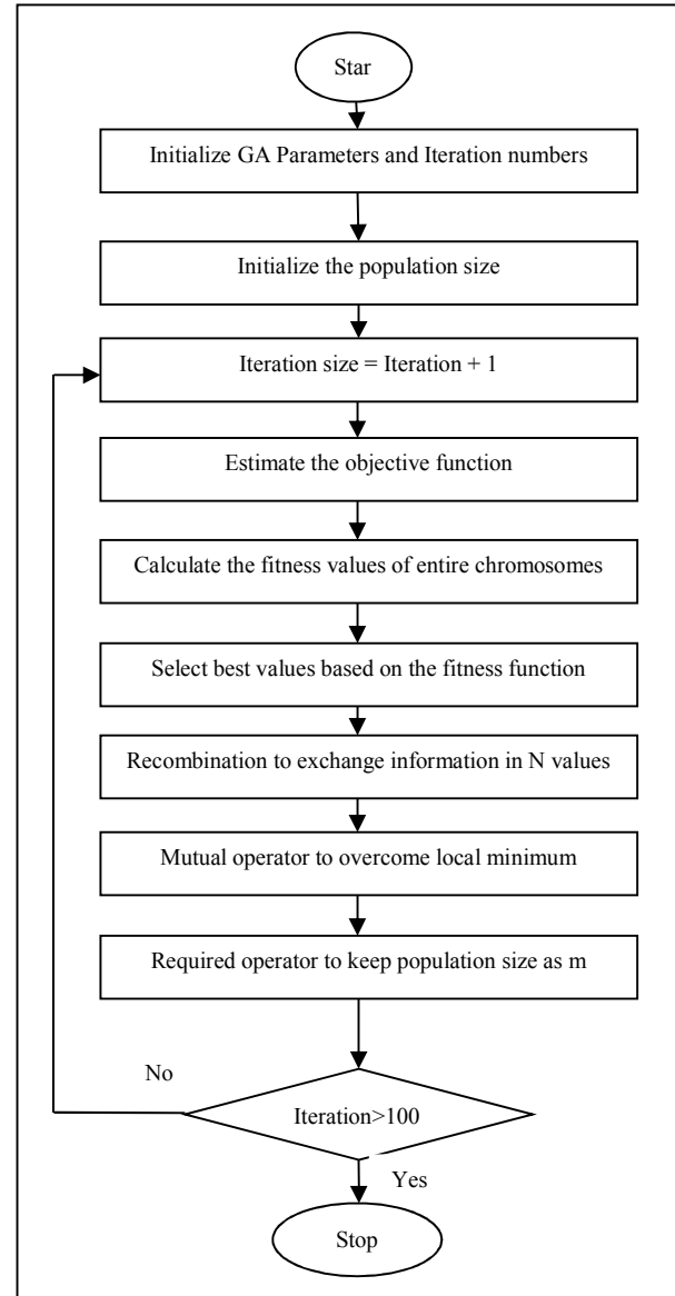
Fig. 5 GA Flow Chart
