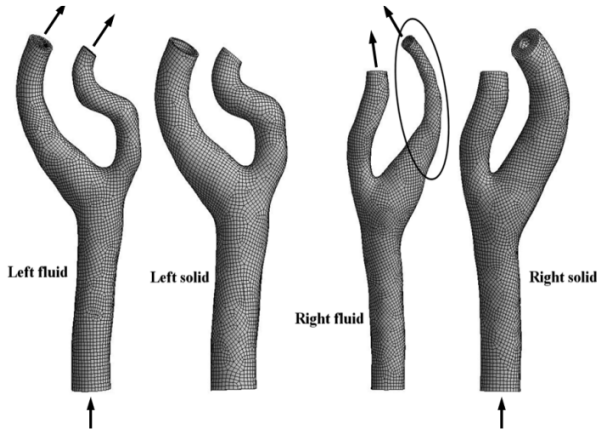
Fig. 3 FSI carotid bifurcation model
