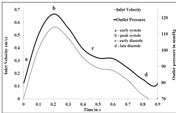
Fig. 4 Flow boundary conditions
