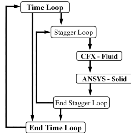
Fig. 1 FSI algorithm
