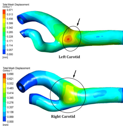
Fig. 8 Comparison of arterial wall displacement contours
