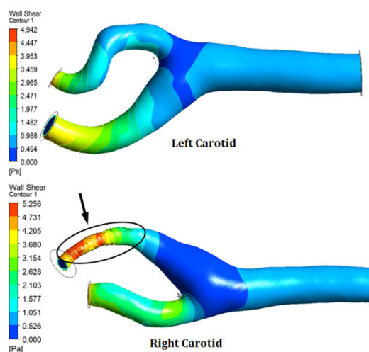
Fig. 6 Comparison of wall shear stress contours
