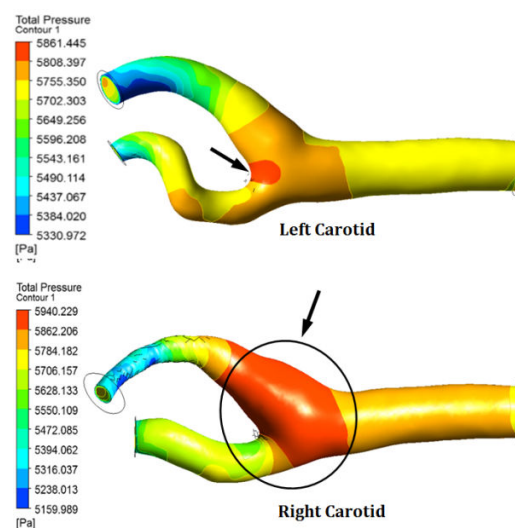
Fig. 7 Comparison of pressure contours
