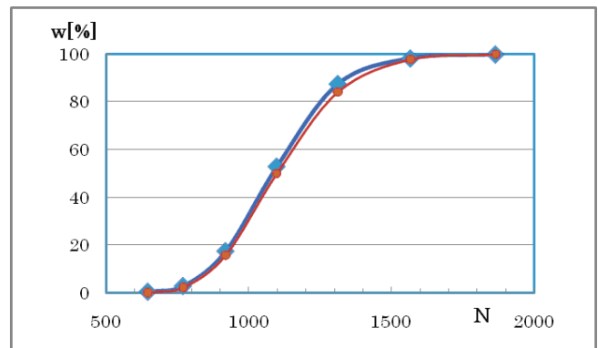
Fig. 4. Comparison of N(w, RL = 2) between theoretical and experimental values at w = 0.1 [%] ( z_0 = 3.0 ), = 2.3 [%] ( z_0 = 2.0 ), ..., = 99.9 [%] ( z_0 = -3.0 ) (◆: experimental value, ●: theoretical value)
