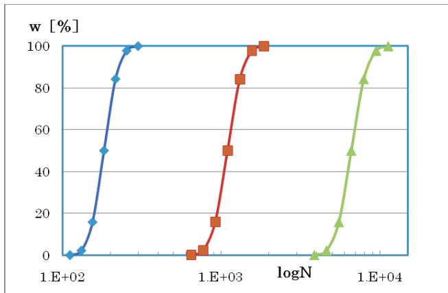
Fig. 3. Theoretical N(w, RL) evaluated by (3) at w = 0.1 [%] ( z_0 = 3.0 ), = 2.3 [%] ( z_0 = 2.0 ), = 15.9 [%] ( z_0 = 1.0 ), = 50.0 [%] ( z_0 = 0.0 ), = 84.1 [%] ( z_0 = -1.0 ), = 97.7 [%] ( z_0 = -2.0 ), = 99.9 [%] ( z_0 = -3.0 ) (◆: RL = 1 , ■: RL = 2 , ▲: RL = 3 )
