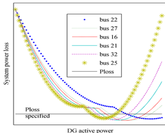
Fig. 1 System power loss variation Vs DG power
