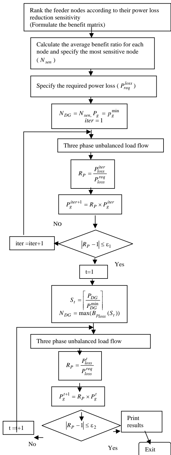
Fig. 2 Flow chart of the proposed heuristic technique
