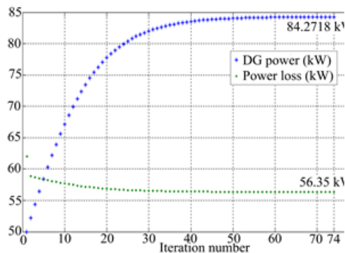
Fig. 5 Convergence characteristics of DG power and power loss
