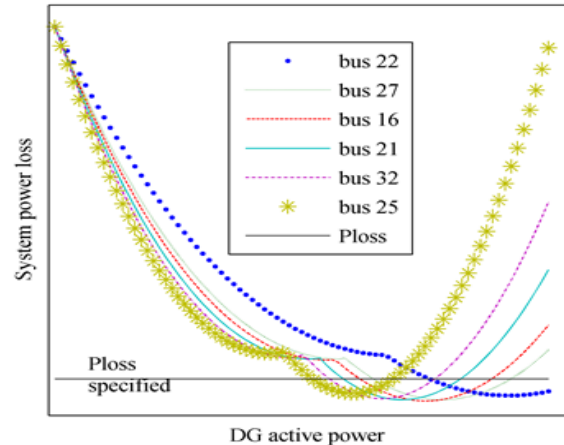
Fig. 1 System power loss variation Vs DG power
