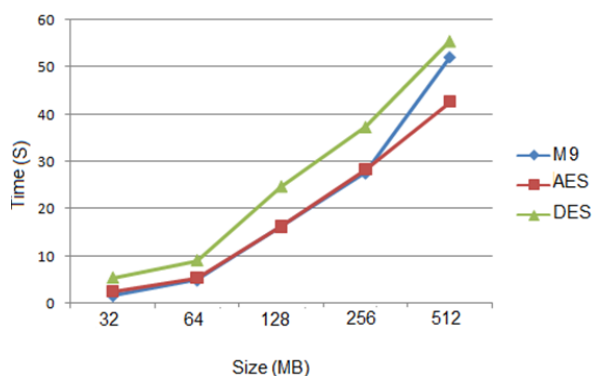
Fig. 8 Response time of AES, DES and M9
