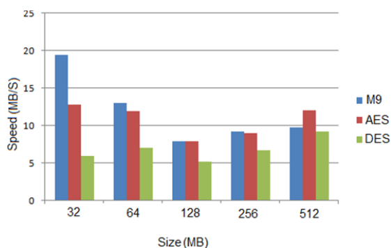
Fig. 9 Speed results of AES, DES and M9
