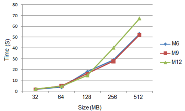
Fig. 6 Response time of M6, M9, and M12
