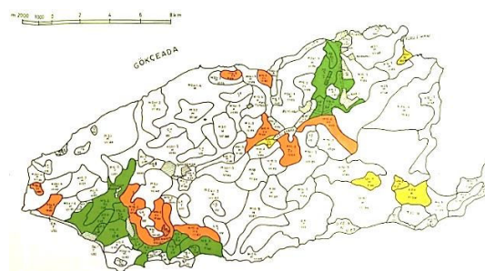
Fig. 4 Soil map of study area
