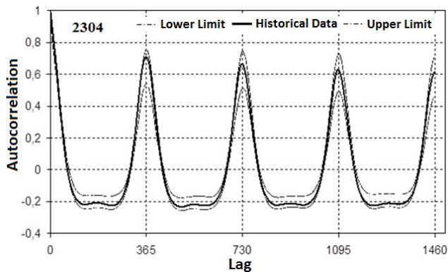
Fig. 5 Correlograms generated by using ARMA (2,2) model for 2304 gauging station with 95% confidence
