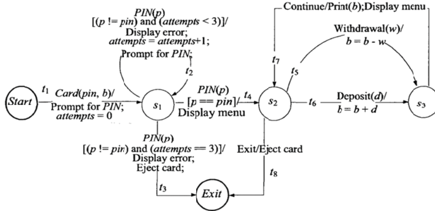
Fig. 1 EFSM model of a simplified ATM system
