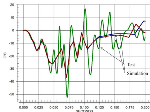
Fig. 18 Accelerations at the left wheel
