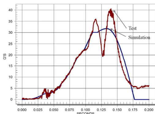
Fig. 21 Accelerations at the passenger head
