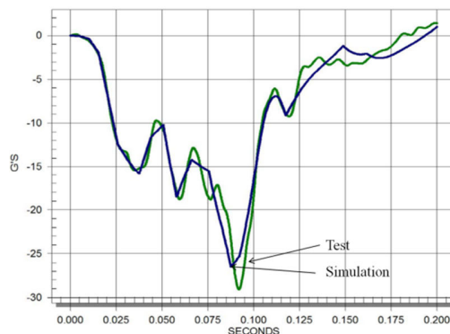
Fig. 17 Accelerations at the engine (Configuration 2)
