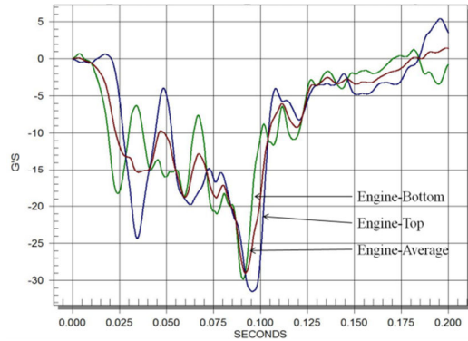
Fig. 5 Accelerations at the engine
