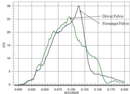
Fig. 9 Accelerations at the dummy pelvis
