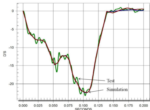
Fig. 14 Accelerations at B-pillar
