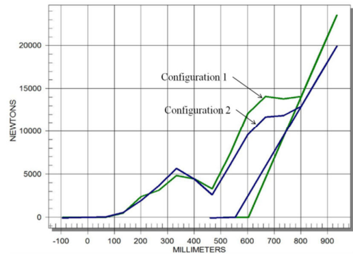
Fig. 11 Load-paths for spring K2
