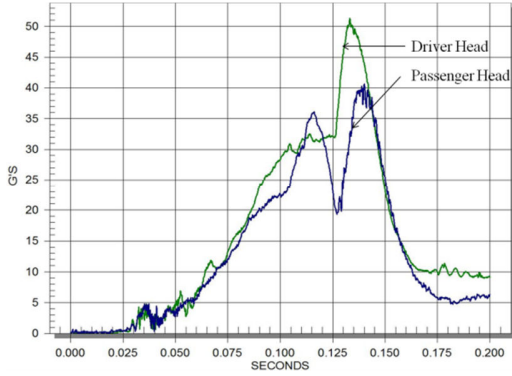
Fig. 7 Accelerations at the dummy head
