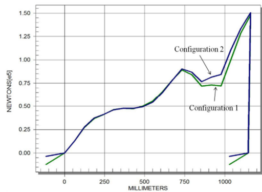
Fig. 10 Load-paths for spring K1
