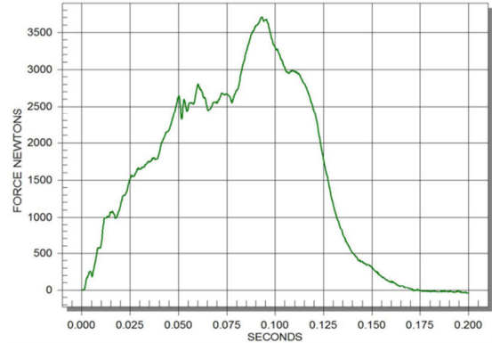
Fig. 3 Barrier force from load cells
