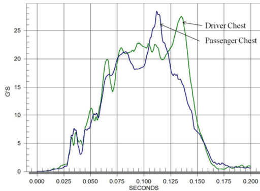
Fig. 8 Accelerations at the dummy chest
