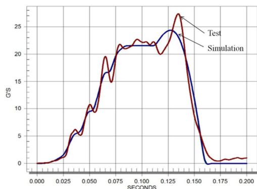
Fig. 22 Accelerations at the driver chest
