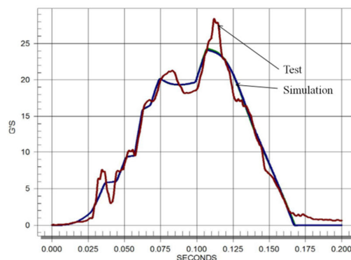
Fig. 23 Accelerations at the passenger chest
