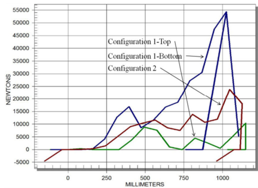
Fig. 12 Load-paths for K6/K11
