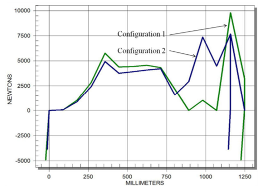
Fig. 13 Load-paths for K14/K9
