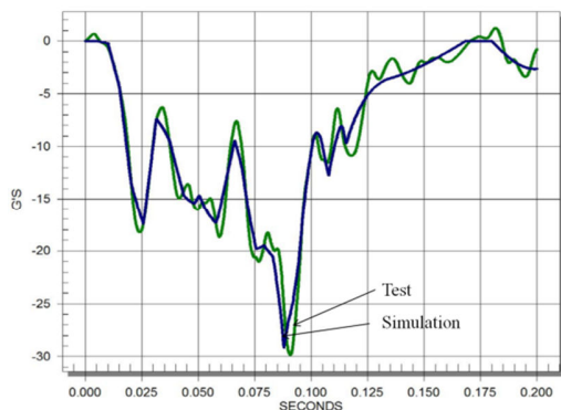
Fig. 16 Accelerations at the engine top (configuration 1)
