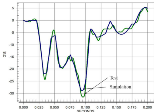
Fig. 15 Accelerations at the engine bottom (Configuration 1)
