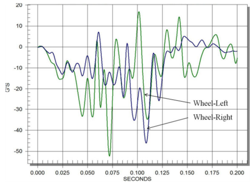
Fig. 6 Accelerations at the wheels L/R
