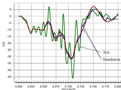
Fig. 19 Accelerations at the right wheel
