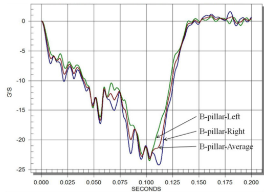
Fig. 4 Accelerations at the B-pillar L/R
