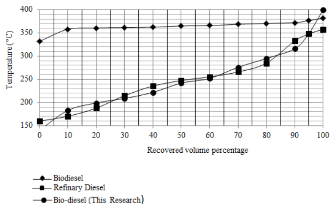
Fig. 2 Distillation Curves of castor oil biodiesel, refinery diesel and bio-diesel
