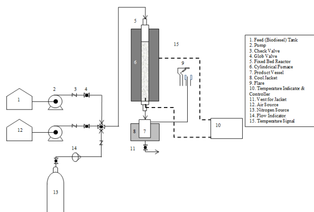
Fig. 1 Continuous thermal cracking system
