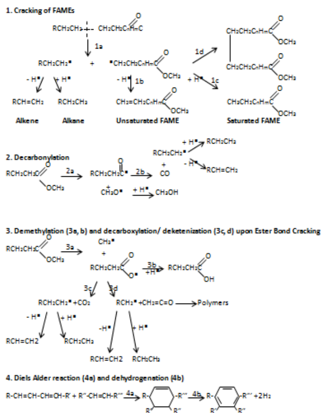
Fig. 3 Thermal decomposition reactions of biodiesel
