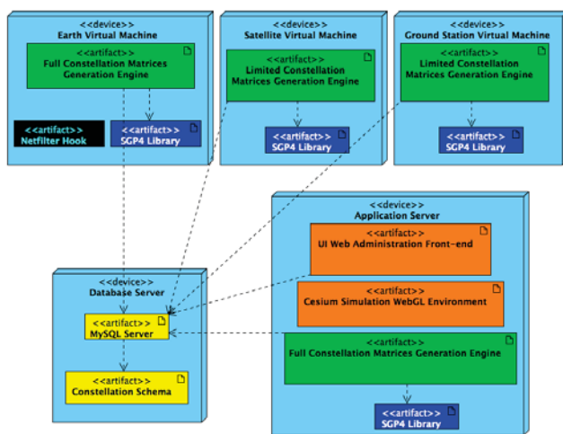
Fig. 5: Framework Deployment Diagram
