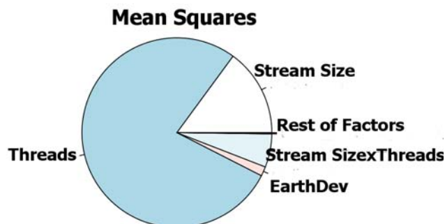
Fig. 8: Factors Mean Squares Ratios
