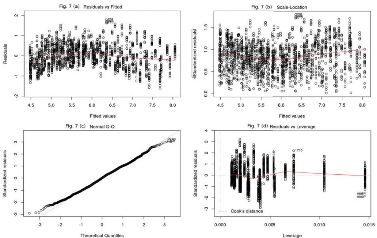
Fig. 7: ANOVA Table and Graph Plots After Normalization
