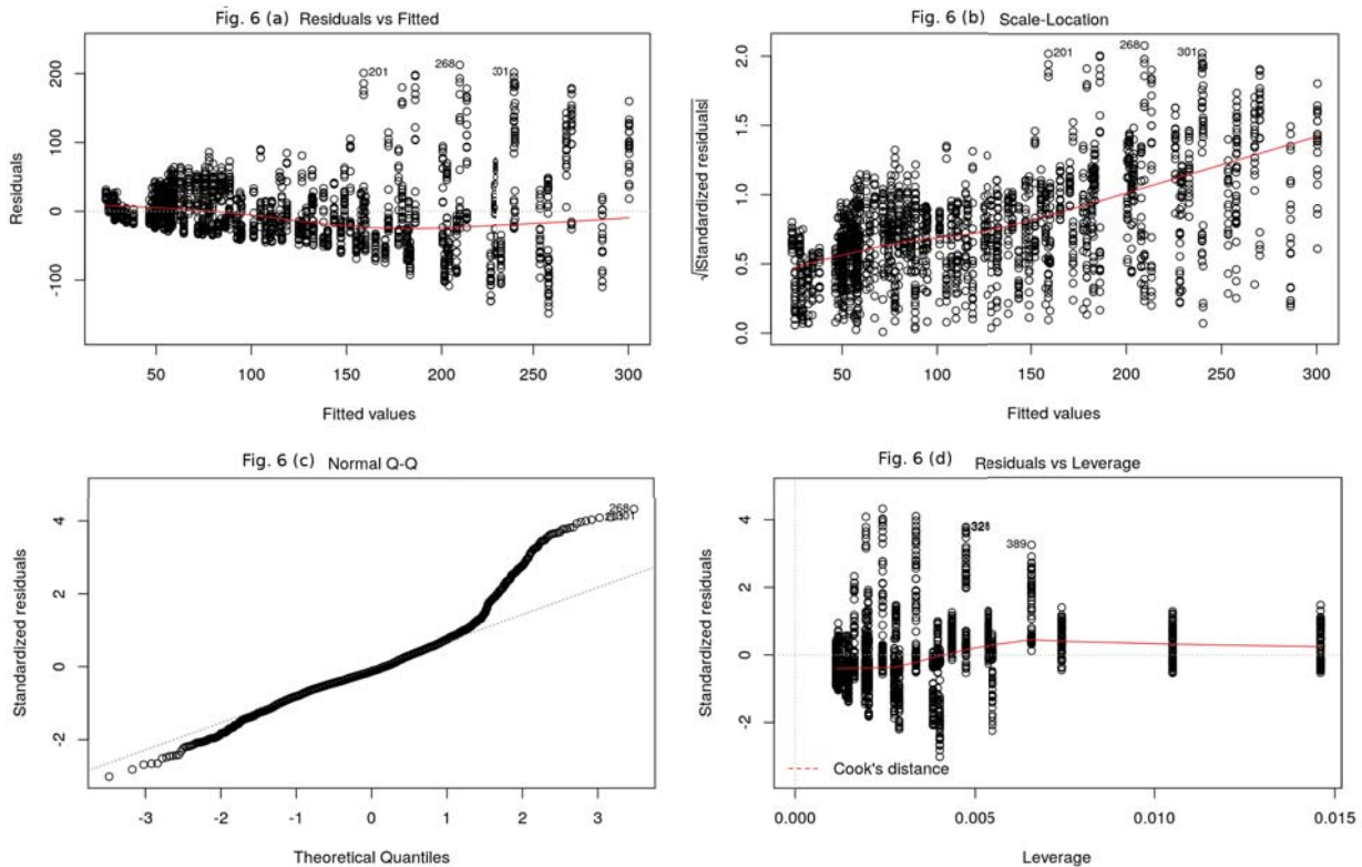
Fig. 6: ANOVA Table and Graph Plots Before Normalization
