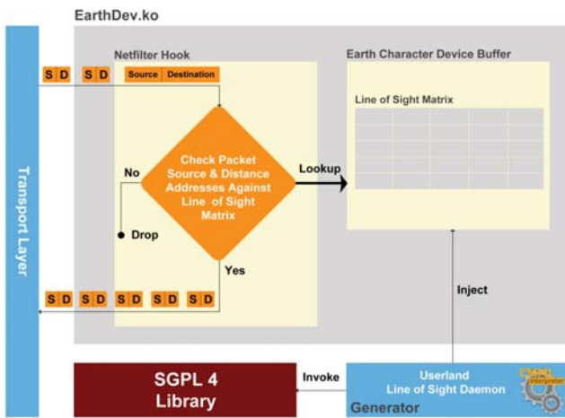
Fig. 3: Simulator Workflow
