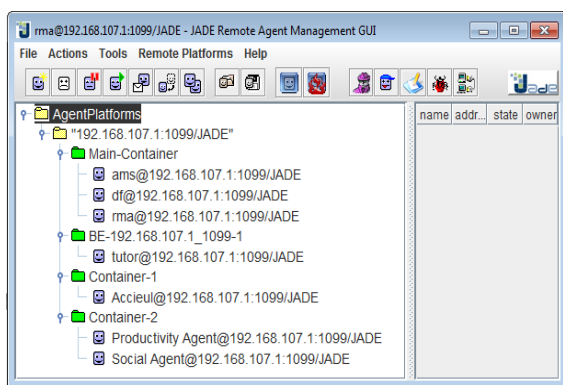
Fig. 7 JADE Remote Agent Management GUI of MASET
