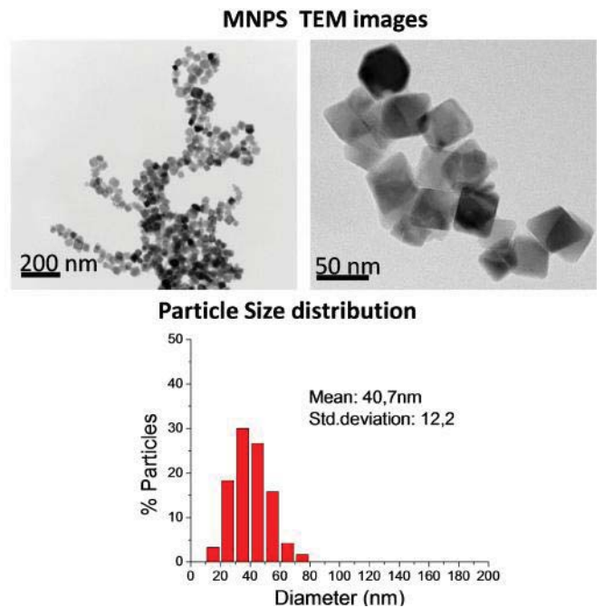
Fig. 6 Transmission electronic microscopy images and particle size distribution for MNPs obtained at the outlet of set-up where mixing was carried out by ultrasonic vibration and reaction stage performed with a gas (N 2 ) segmented flow. Reaction stage: 100°C and 360 s
