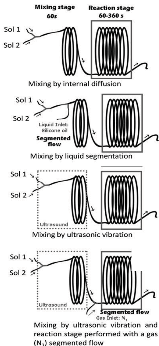
Fig. 1 Schemes of the microfluidics set-up designed to produce MNPs in continuous flow
