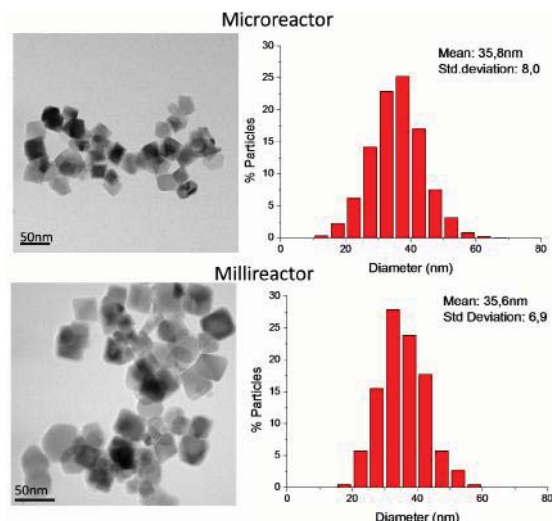
Fig. 9 TEM micrographs and particle-size distribution of MNPs produced in a micro and a millireactor under ultrasonic radiation and \text{N}_2 gas-liquid segmented flow: residence time and synthesis temperature were 6 min and 90°C, respectively
