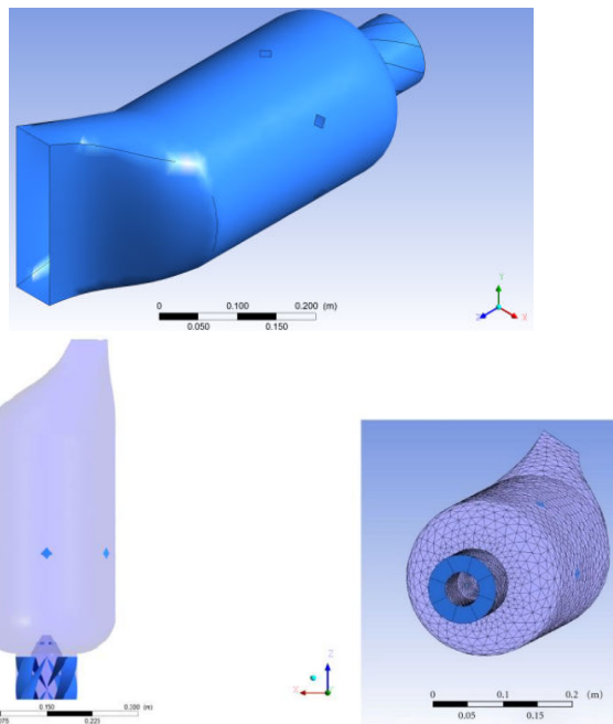
Fig. 1 Combustor Geometry Model and Mesh
