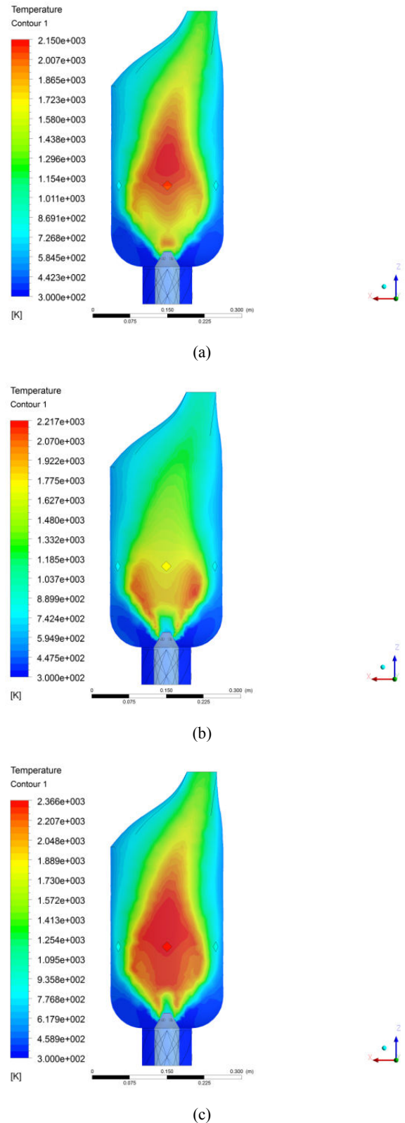
Fig. 2 Contours of Temperature (a) Natural gas, (b) Syngas (PKS+30%PE) and (c) Hydrogen
