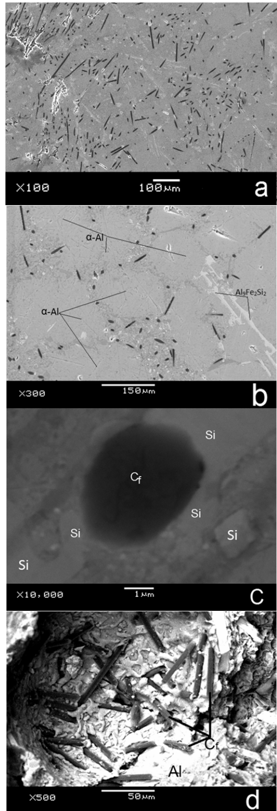
Fig. 2 Microstructure of successful A356/ C_{sf} composite showing random orientation of fibers in the aluminum matrix (a) \times 100 , (b) \times 300 , microstructure of interface of C_{sf} and aluminum matrix (c), Fractured surface of composite which shown fibers in matrix (d)
