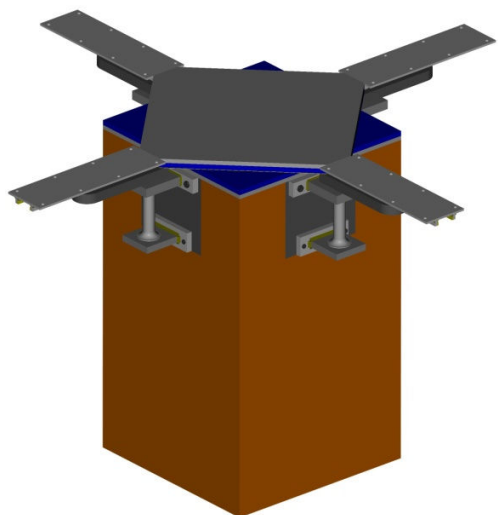
Fig. 8 MARTI, an integrated bearing-damper isolation system
