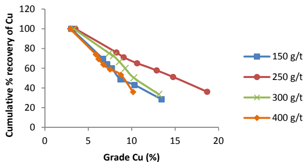
Fig. 3 (b) Cu cumulative % recovery against cumulative concentrate mass (g) and grade (%)
