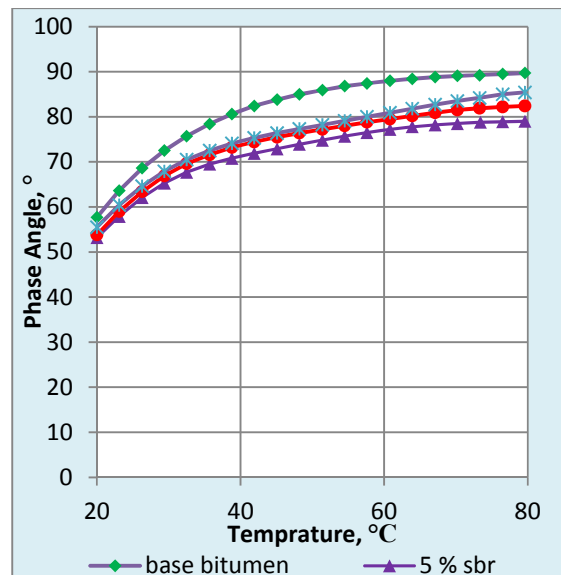
Fig. 3 Phase angle of base bitumen and modified ones by using SBR
