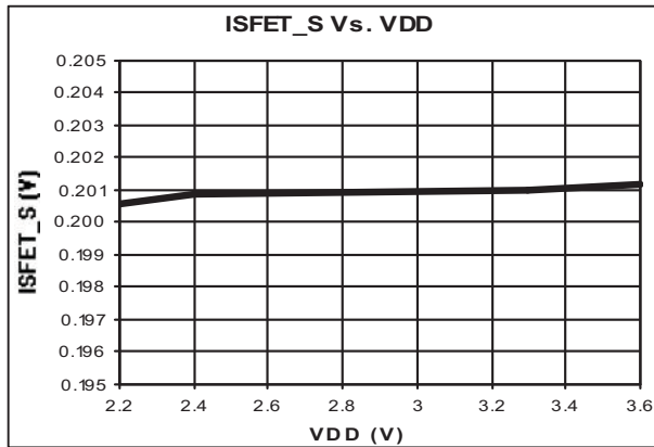
Fig. 13 Measured voltages for source of ISFET with varies supply voltage. © 2011 MIMOS Berhad
