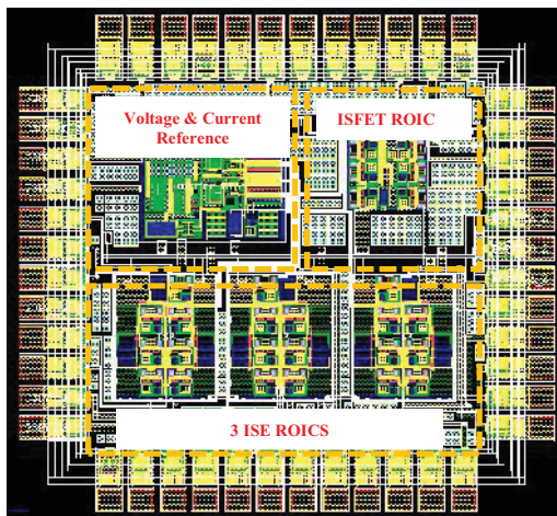
Fig. 5 Physical layout of ISFET and ISE readout circuits. © 2011 MIMOS Berhad
