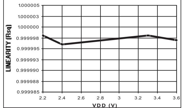
Fig. 10 Output linearity of ISFET readout circuit with different supply voltages. © 2011 MIMOS Berhad
