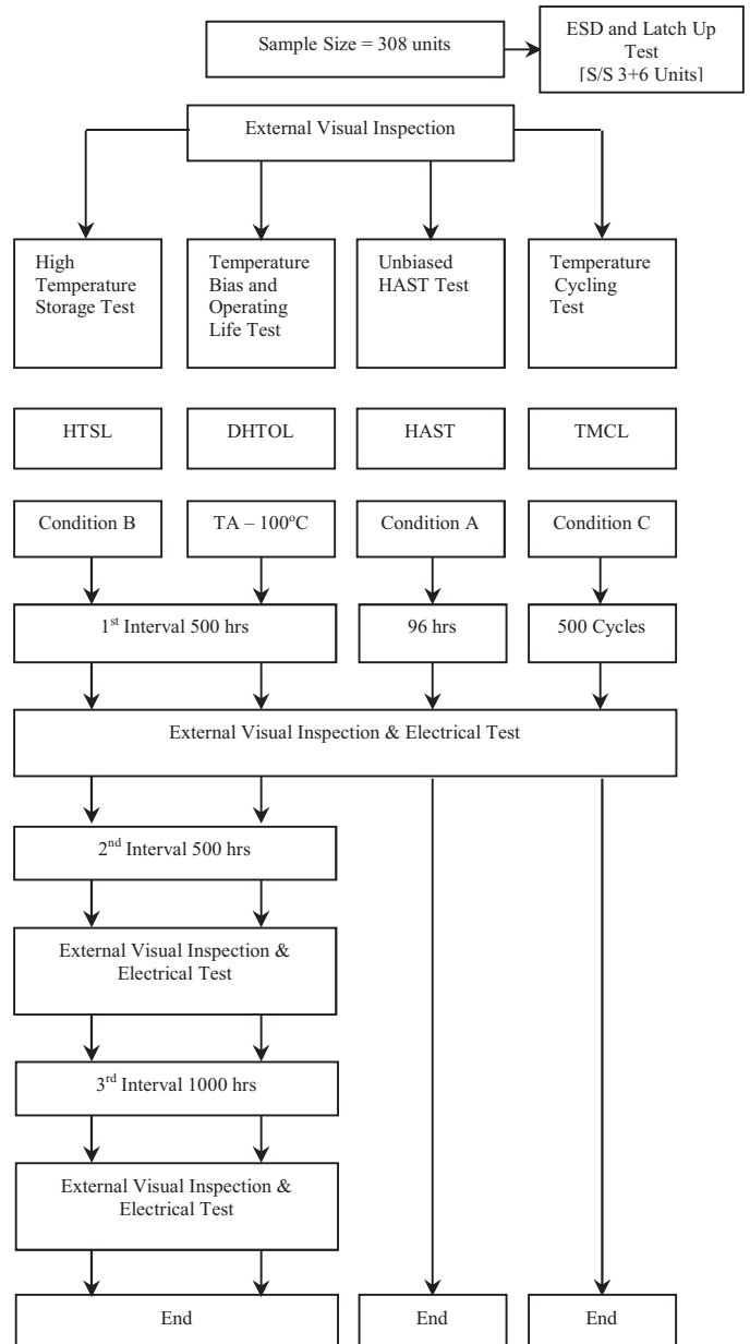
Fig. 14 Flow diagram of reliability test
