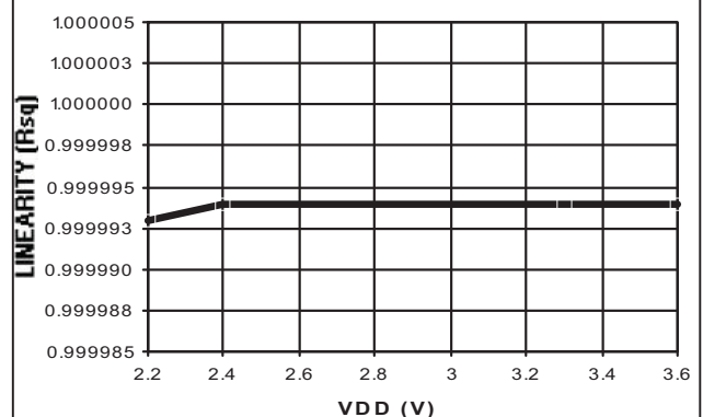
Fig. 11 Output linearity of ISE readout circuit with different supply voltages. © 2011 MIMOS Berhad
