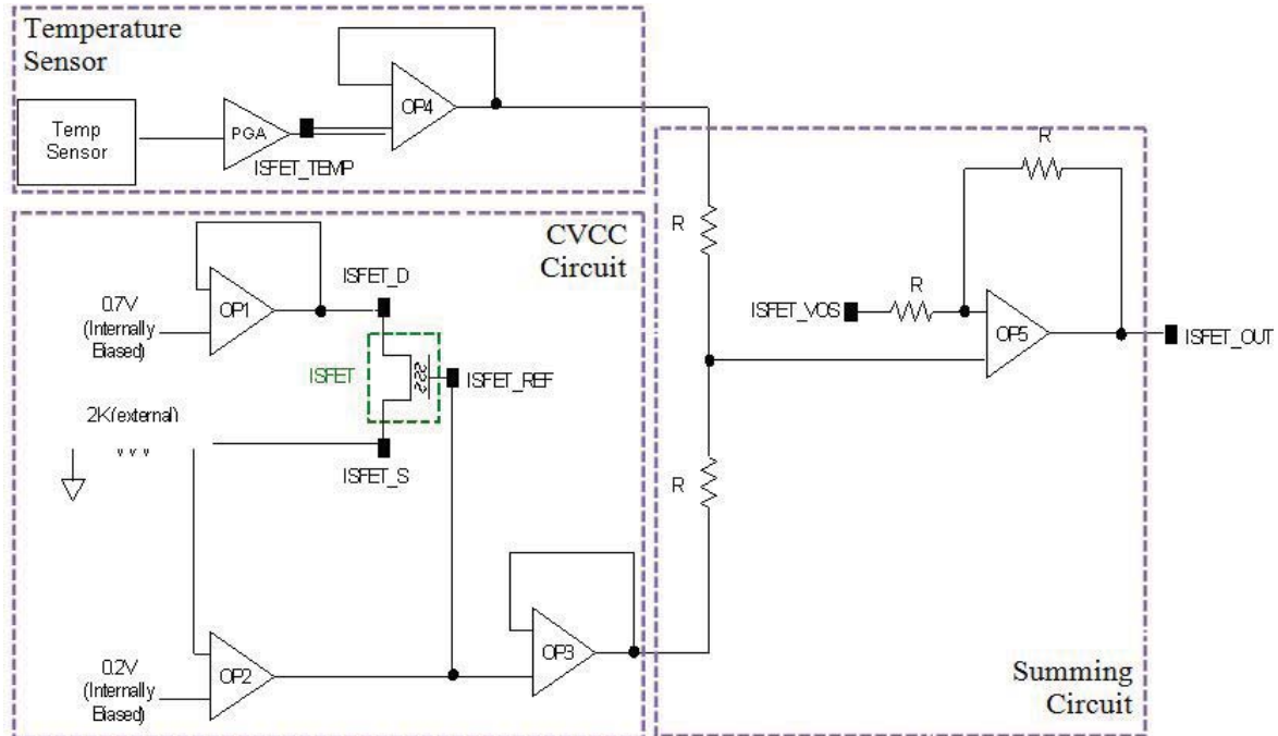
Fig. 4 Readout interface circuit for ISFET based sensor
