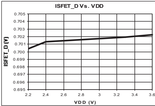
Fig. 12 Measured voltages for drain of ISFET with varies supply voltage. © 2011 MIMOS Berhad
