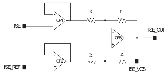
Fig. 3 Read-out interface circuit for ISE based sensor
