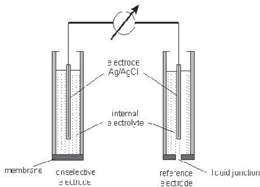
Fig. 2 Operational principle of an ISE
