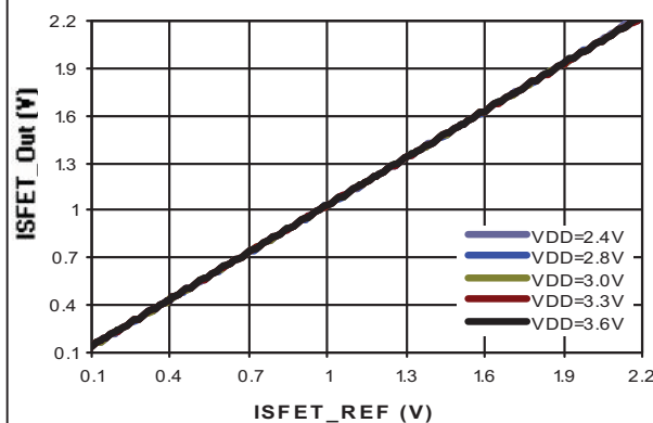
Fig. 8 Output voltage of ISFET readout circuit with different supply voltages. © 2011 MIMOS Berhad
