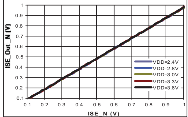
Fig. 9 Output voltage of ISE readout circuit with different supply voltages. © 2011 MIMOS Berhad
