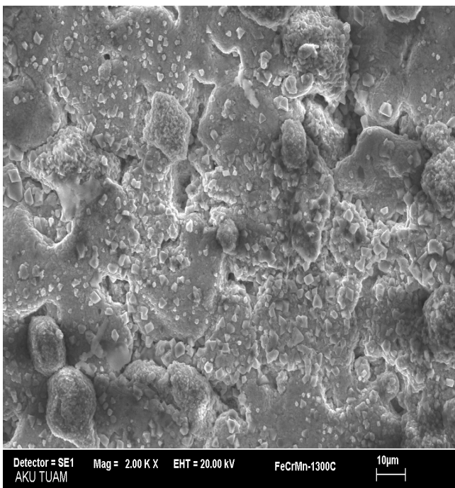
Fig. 4 SEM view of Fe-Cr-Mn composite 1300°C
