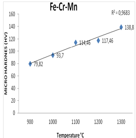
Fig. 2 The micro hardness tests results from sintered specimens treated at different temperatures
