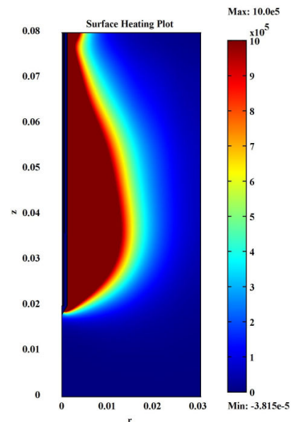
Fig. 4 Surface heating plot of Unchoked antenna in the tissue, 2D mode
