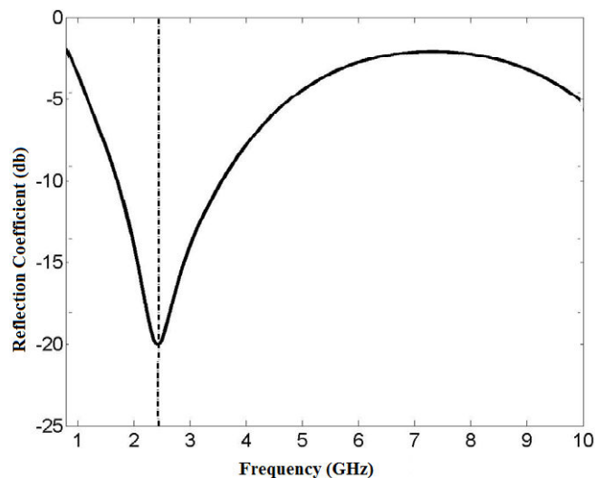
Fig. 7 The simulated reflection coefficient of the choked antenna, expressed logarithmically. The dashed line represents the commonly used MWA frequency of 2.45 GHz.
