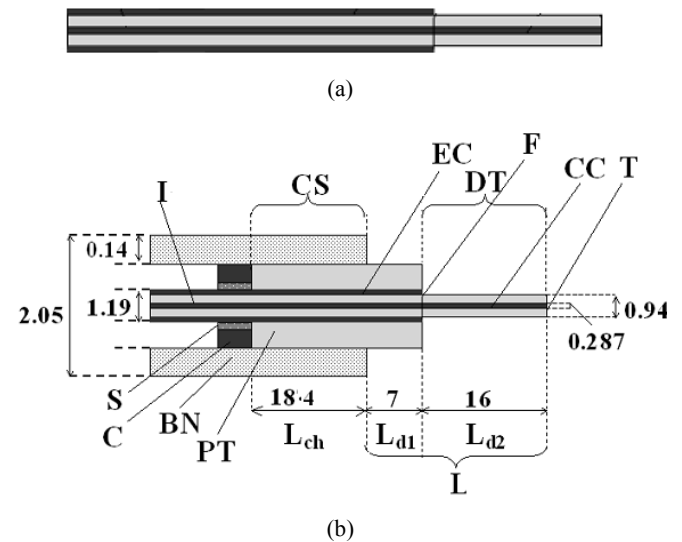
Fig. 1 (a) Cross section of a conventional unchoked antenna (b) Cross section of a conventional choked antenna of Legend: EC=CC = external/central coaxial conductor (copper), I = insulator (P.T.F.E.), PC = plastic catheter (e.g., silicone), CS = choke section, F = antenna feed, T = antenna tip, DT =dielectric tip, BN = biopsy needle, C = copper collar, S = solder, PT = plastic tubing (P.T.F.E.), L = length of CS, L = distance between CS input and T, L = distance between CS input and F, L = length of DT; all sizes are in mm
