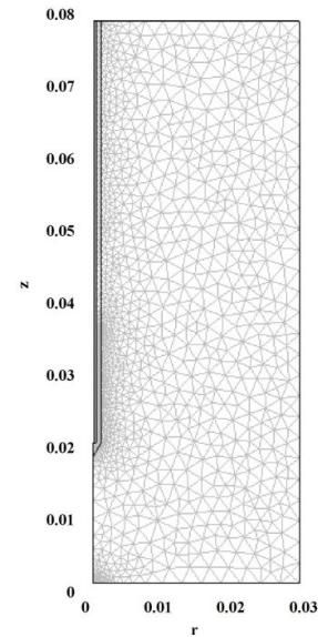
Fig. 3 Meshing for Choked antenna
