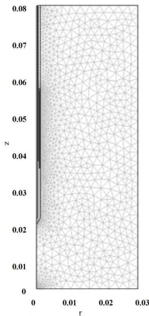
Fig. 2 Meshing for Unchoked antenna
