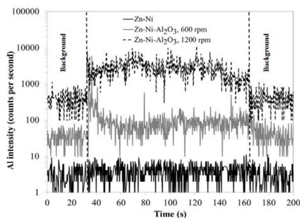
Fig. 2 LA-ICP-MS results of Al for Zn-Ni-Al 2 O 3 coatings deposited at two agitation speeds. Analysis from Zn-Ni alloy is also shown for comparison
