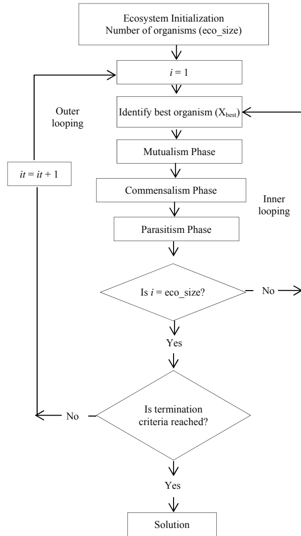
Fig. 1 SOS Algorithm Procedure
