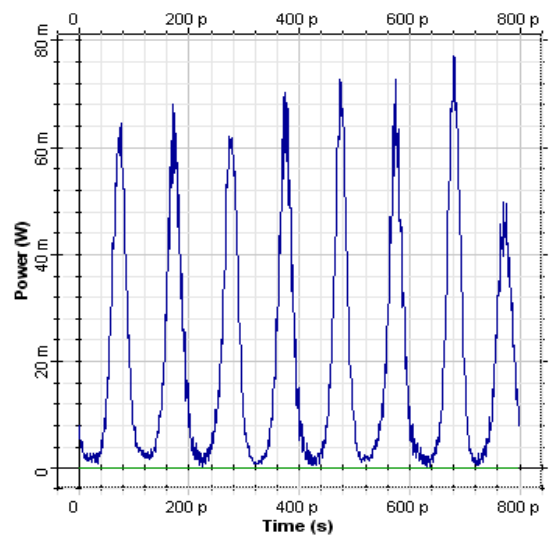
Fig. 11 (b) Time domain analyzer view of pulse sequence received at the end of 200 Km fiber length implemented in soliton system
