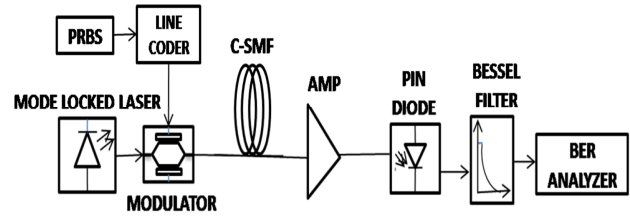
Fig. 1 Skeletal view of basic telecommunication model
