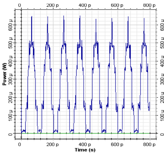
Fig. 9 (a) Time domain analyzer view of bit patterns in conventional transmission system
