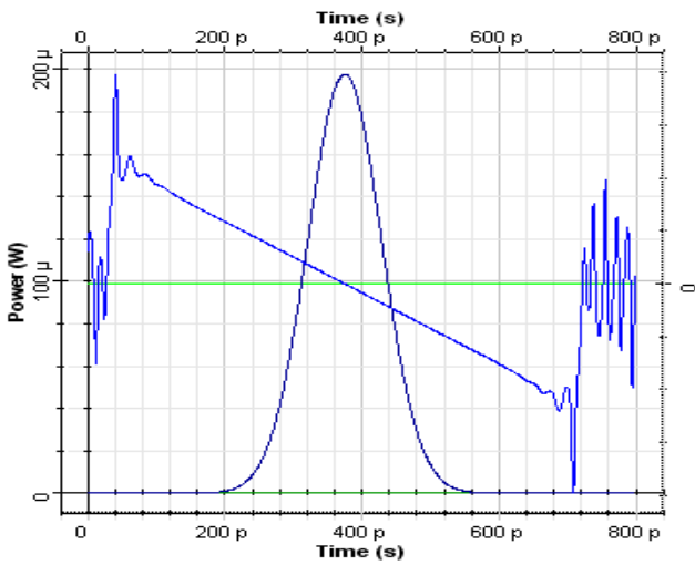
Fig. 6 (a) Time domain analyzer view of Gaussian pulse received at the end of 5L_D=56.35 Km
