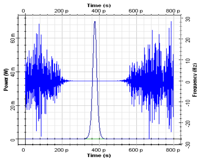
Fig. 3 (a) Analysis of hyperbolic-secant pulse approximating soliton system before fiber
