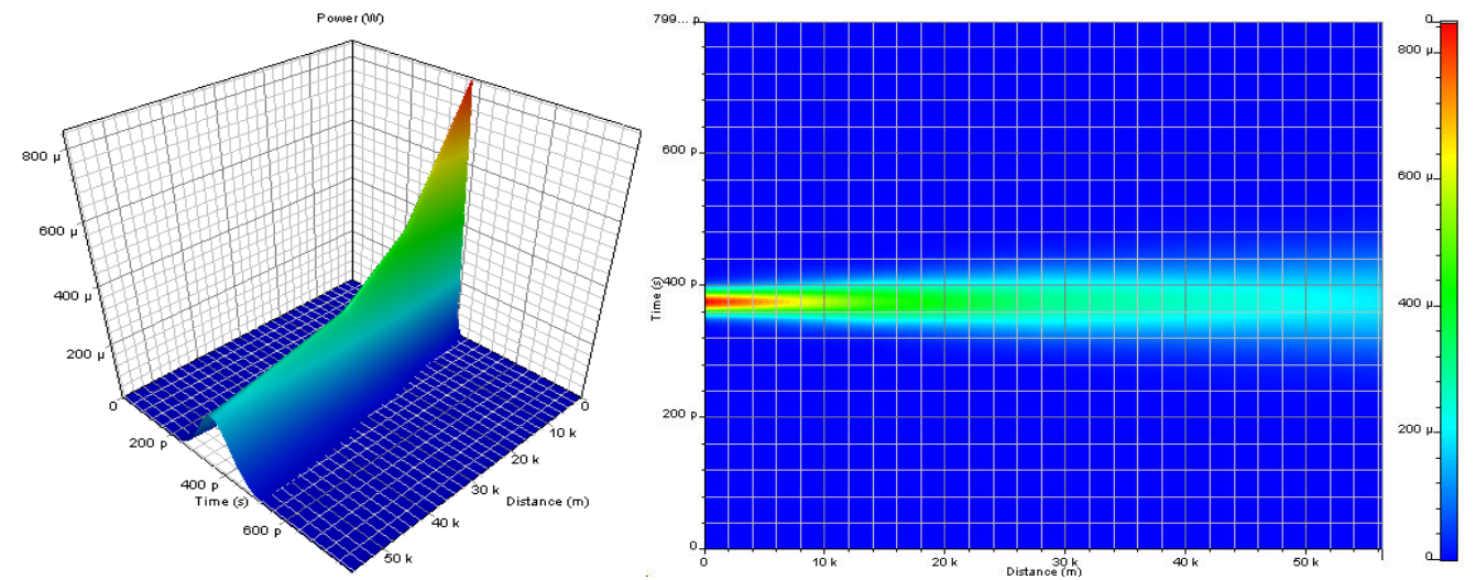
Fig. 5 (a) 3D view of Gaussian pulse received at the end of five dispersion length, 5L_D=56.35\text{Km}
