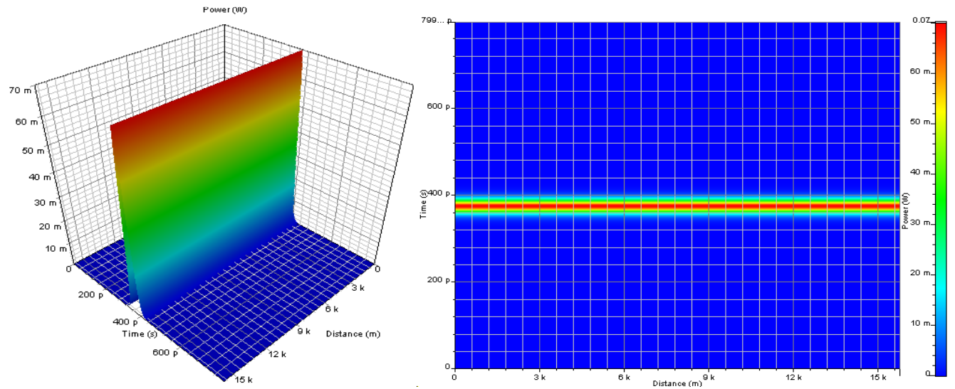
Fig. 4 (b) 3D view of soliton pulse at the end of one soliton period, z_0=15.79\text{ Km}
