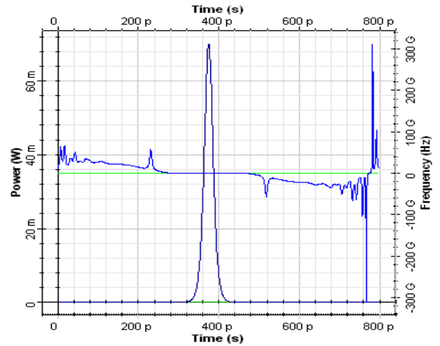
Fig. 6 (b) Time domain analyzer view of Hyperbolic secant pulse received at the end of 5z_0=78.95
