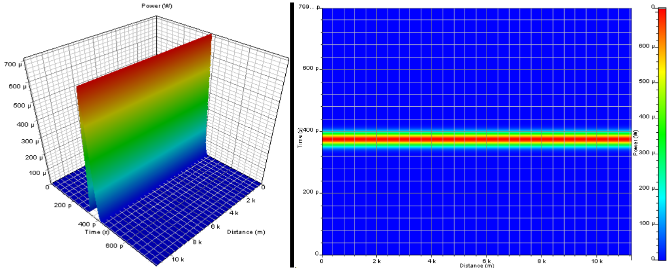
Fig. 4 (a) 3D view of Gaussian pulse received at the end of one dispersion length, L_D=11.27\text{Km}
