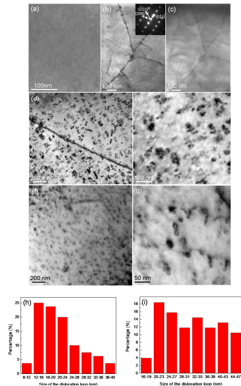
Fig. 3 Low magnification TEM micrographs showing the microstructures of the specimens (a) un-irradiated condition of Fe-0.2wt.%V alloy; (b) bright-field TEM image (c) dark-field TEM image of the irradiated Fe-0.2wt.%V alloy, the up inset of (b) is the corresponding SAED pattern; (d) dislocation loops in the irradiated Fe-0.2wt.%V alloy; (e) enlarged part of (d); (f) general views of the detailed arrangement of dislocations in the irradiated pure Fe; (g) enlarged part of (f); (h) and (i) showing the size distribution of the dislocation loops in Fe-0.2wt.%V alloy and pure Fe, respectively
