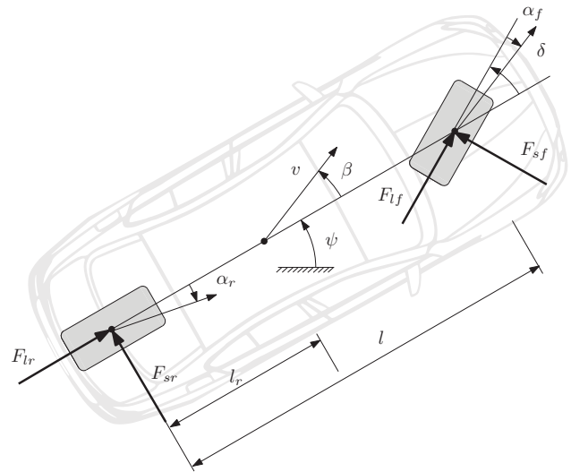
Fig. 9. Single-track model
