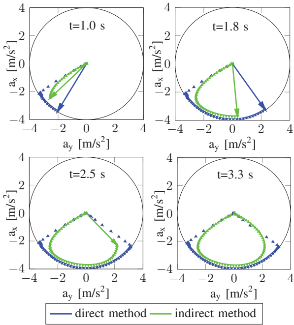
Fig. 8. Kamm's circle for the evasion maneuver
