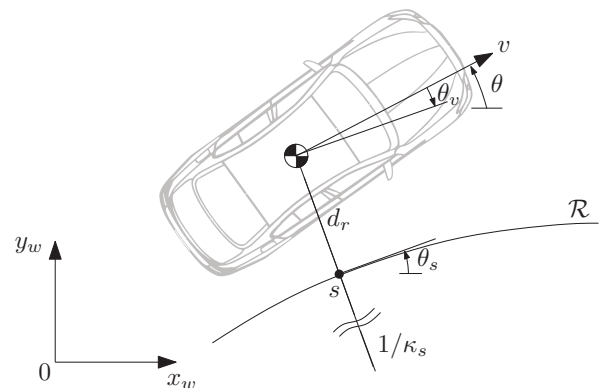
Fig. 1. Vehicle relative to a road \mathcal{R} in world coordinates (x_w, y_w)
