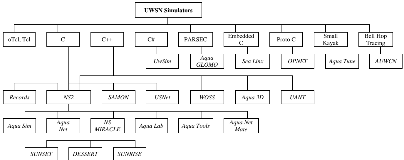
Fig. 2 UWSN Taxonomy
