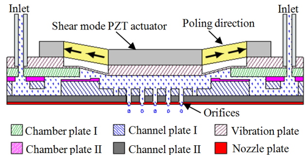
Fig. 3 The cross section view for the microdroplet ejector
