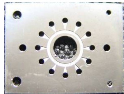
Fig. 8 The fabricated nickel chamber plate II
