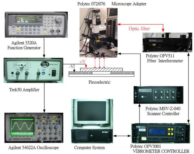
Fig. 19 Configuration of instruments for measuring the actuated displacement of the shear mode piezoelectric actuator
