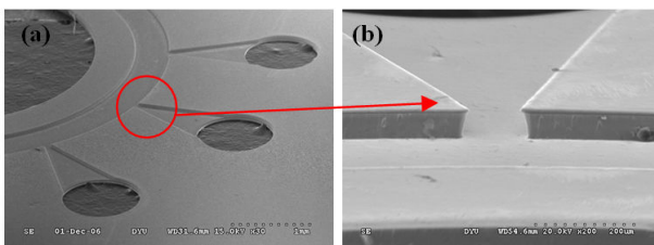
Fig. 11 SEM picture of the nickel chamber plate II (a) and close-up view of the diffuser channel (b)
