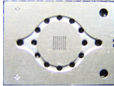
Fig. 14 The fabricated stainless steel bottom view of channel plate I
