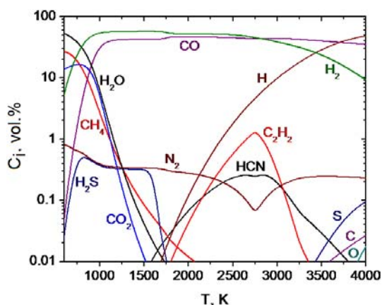
Fig. 1 Temperature dependence of the organic component concentration in the gaseous phase during comprehensive coal processing
