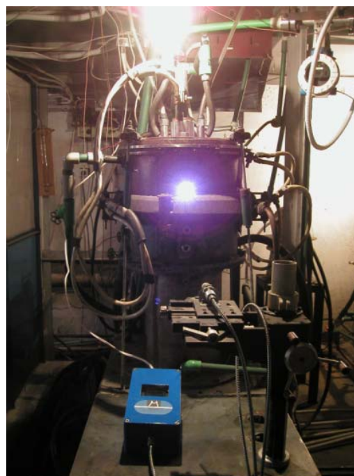
Fig. 7 The plasma chemical reactor in operation
