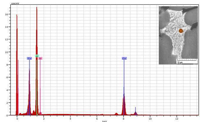
Fig. 7 The Al-Al 2 Cu-Si phase identification using EDX point analysis, etch. 0.5 % HF
