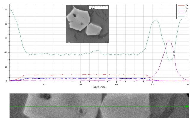
Fig. 9 The Al_{15}(FeMnCr)_3Si_2 identification using phase line EDX analysis, etc. 0.5 % HF
