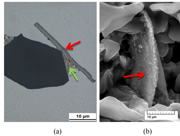
Fig. 4 The Fe-rich intermetallic phases Al_3FeSi in secondary AlSi9Cu3 cast alloy, as-cast state; (a) Al_3FeSi needles; (b) Al_3FeSi platelets- SEM
