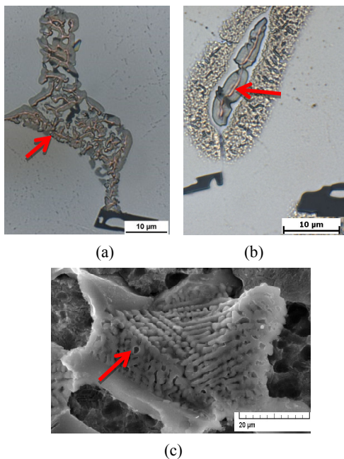
Fig. 3 The Cu-rich intermetallic phases in secondary AlSi9Cu3 cast alloy, as-cast state; (a) Al-Al 2 Cu-Si; (b) Al_2Cu ; (c) SEM-Al-Al 2 Cu-Si
