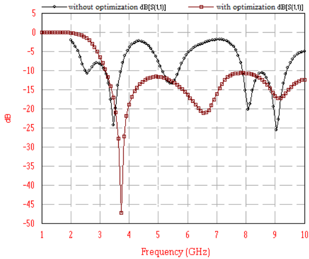
Fig. 5 Comparison of s-parameters with and without optimization
