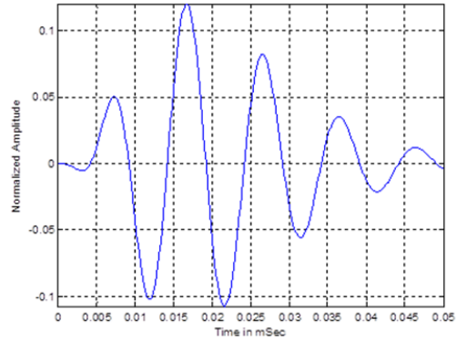
Fig. 6 Gammatone L_2 Normalized Impulse Responses, atom1 = 100Hz
