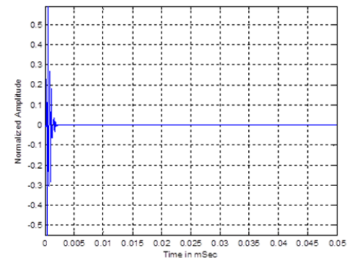
Fig. 8 Gammatone L_2 Normalized Impulse Responses, atom16 = 3200Hz
