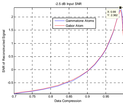
Fig. 12 Matching Pursuit Reconstruction SNR Verses Data Compression for a -2.5dB SNR
