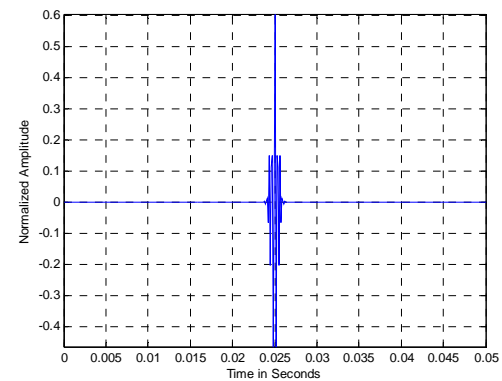
Fig. 7 Gabor L_2 Normalized Impulse Responses, atom16 = 3200Hz
